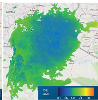
Remote sensed and modelling signals in the Nyanza/Winam Gulf
