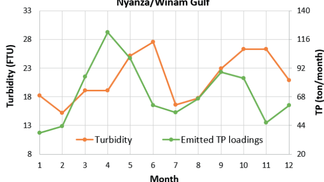
Remote sensed and modelling signals in the Nyanza/Winam Gulf
