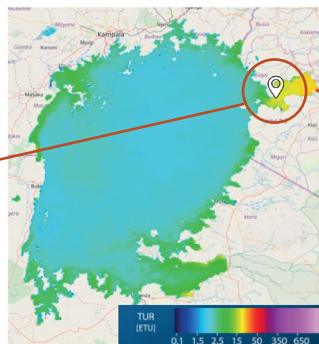
Remote sensed and modelling signals in the Nyanza/Winam Gulf
